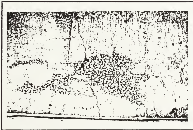
Figure 2.13 Surface Honeycombing (Reference 3)
